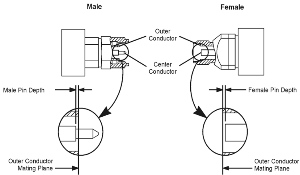
Figure 3-1 Pin depth for a 3.5mm connectors
