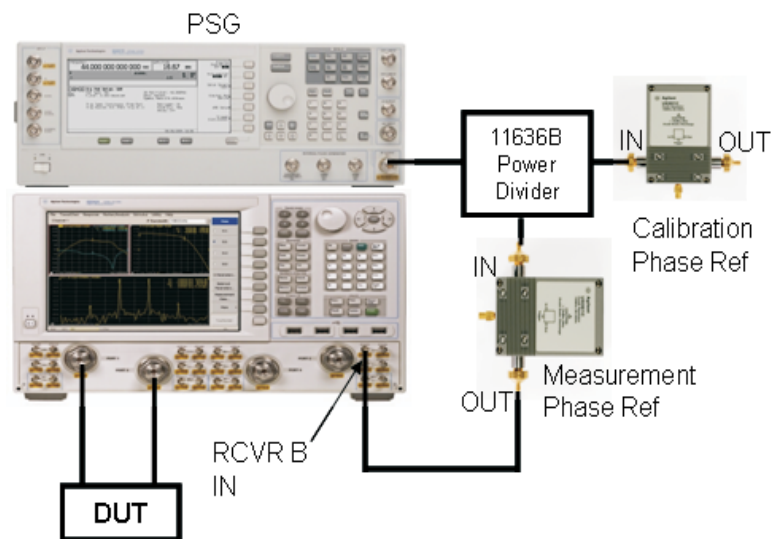
Figure 2-1 U9391C Comb Generator and PNA-X Configuration
