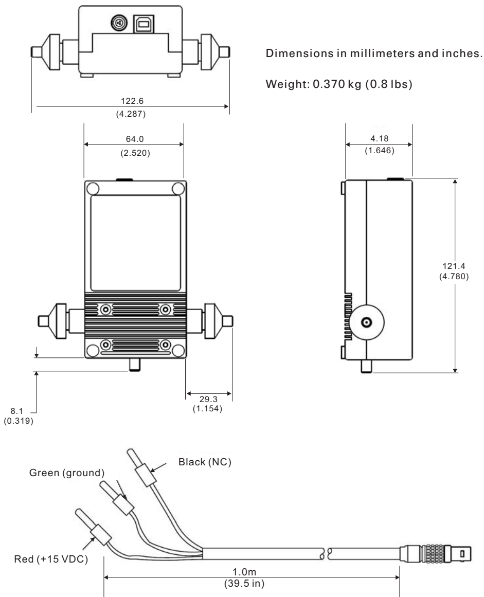
Figure 3-2 Mechanical Dimension of U9391C Comb Generator
