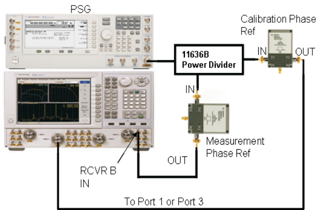
Figure 4-2 Quick-check Configuration for NVNA Test
